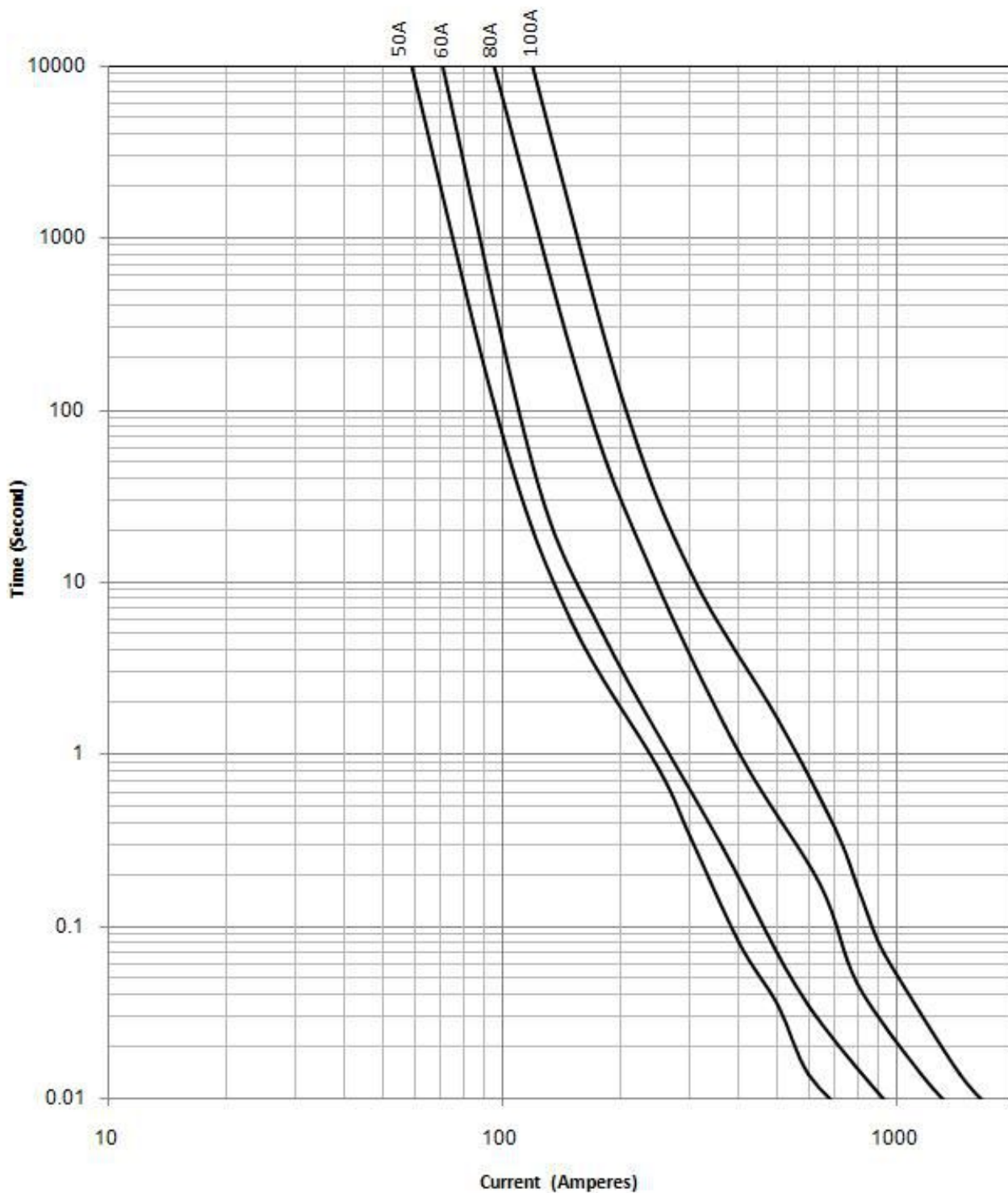
Time-Current Curve 时间电流曲线
